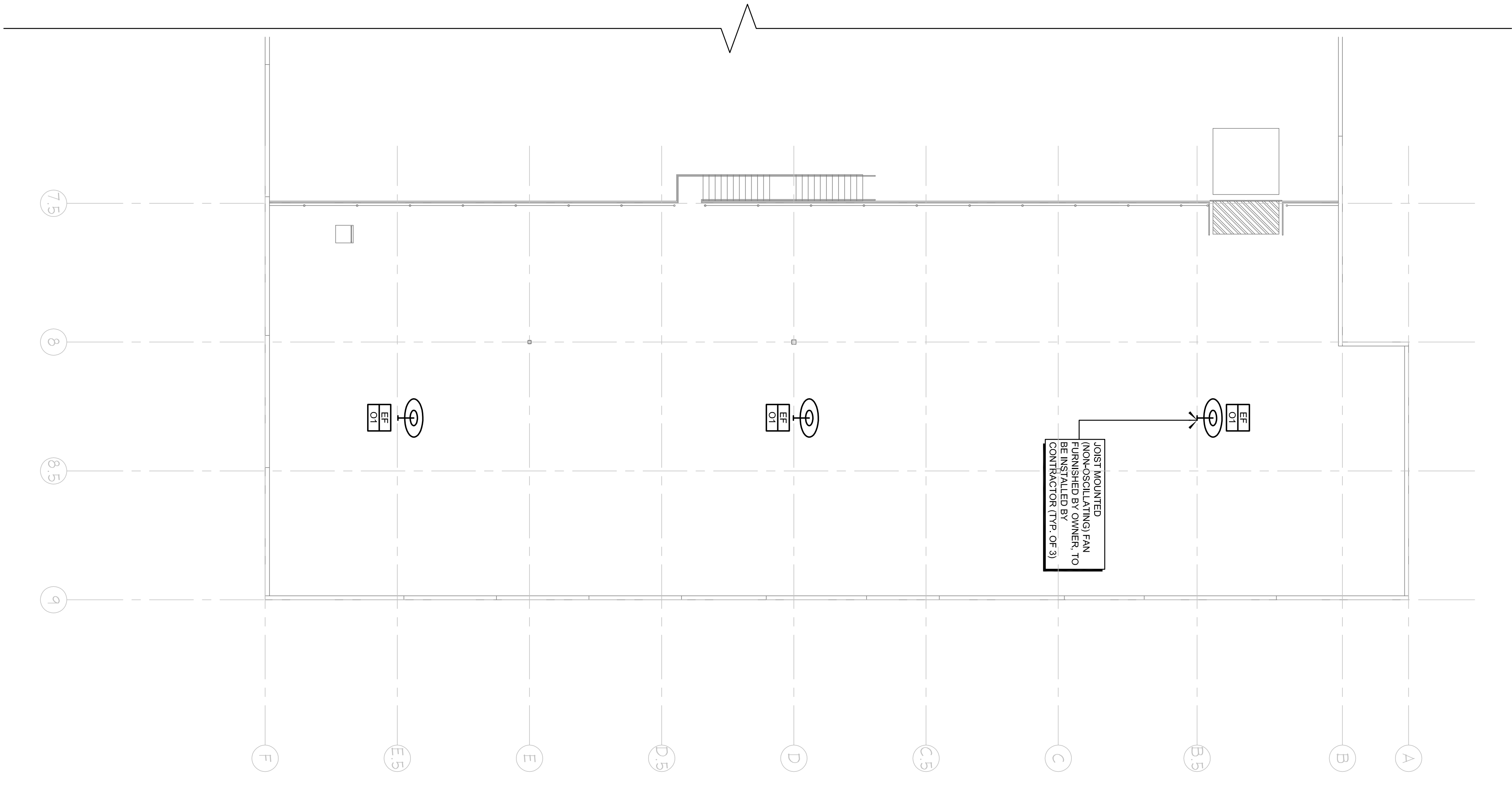
MEZZANINE PLAN - MECHANICAL SCALE: 3/32" = 1'-0"
