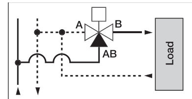
Normally closed actuator
