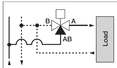
Installed on the supply in diverting configuration
